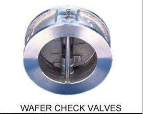
WAFER CHECK VALVES SIZES 1 1/2" - 36" PRESSURES 150 ENDS FLANGED
